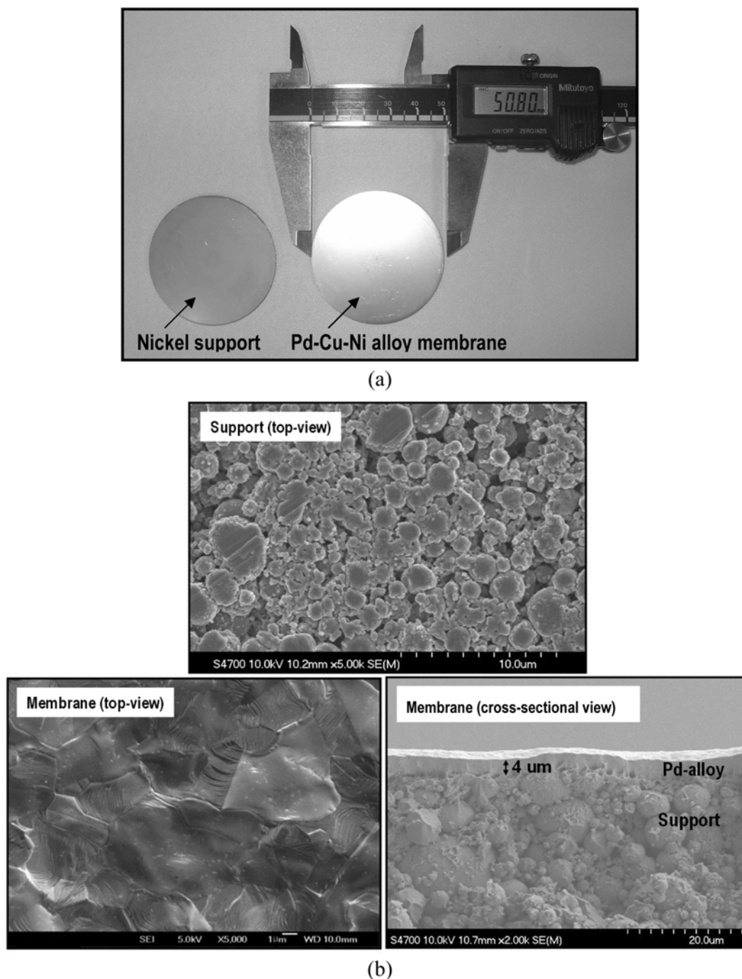
Fig. 3. Photographs and SEM images of the porous nickel support and Pd-alloy membrane.
